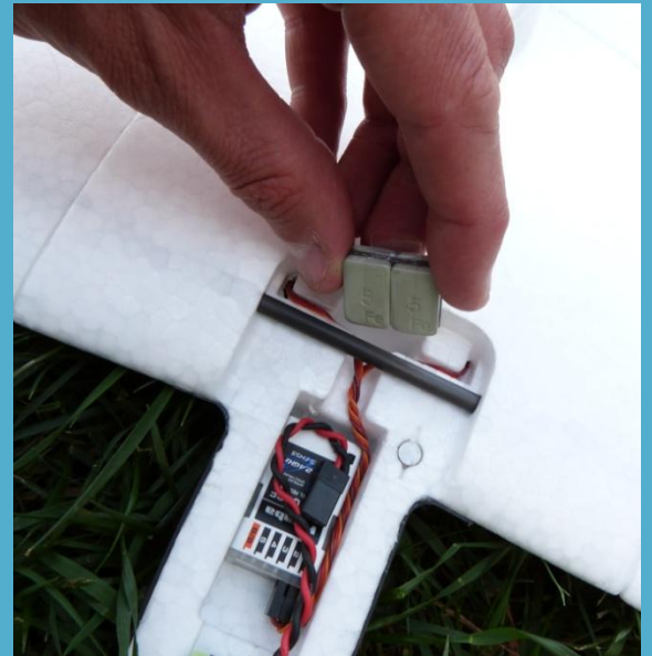
If the wind comes up, you will be ready! Quickly add or remove ballast from the Alula-TREK depending on the conditions.
