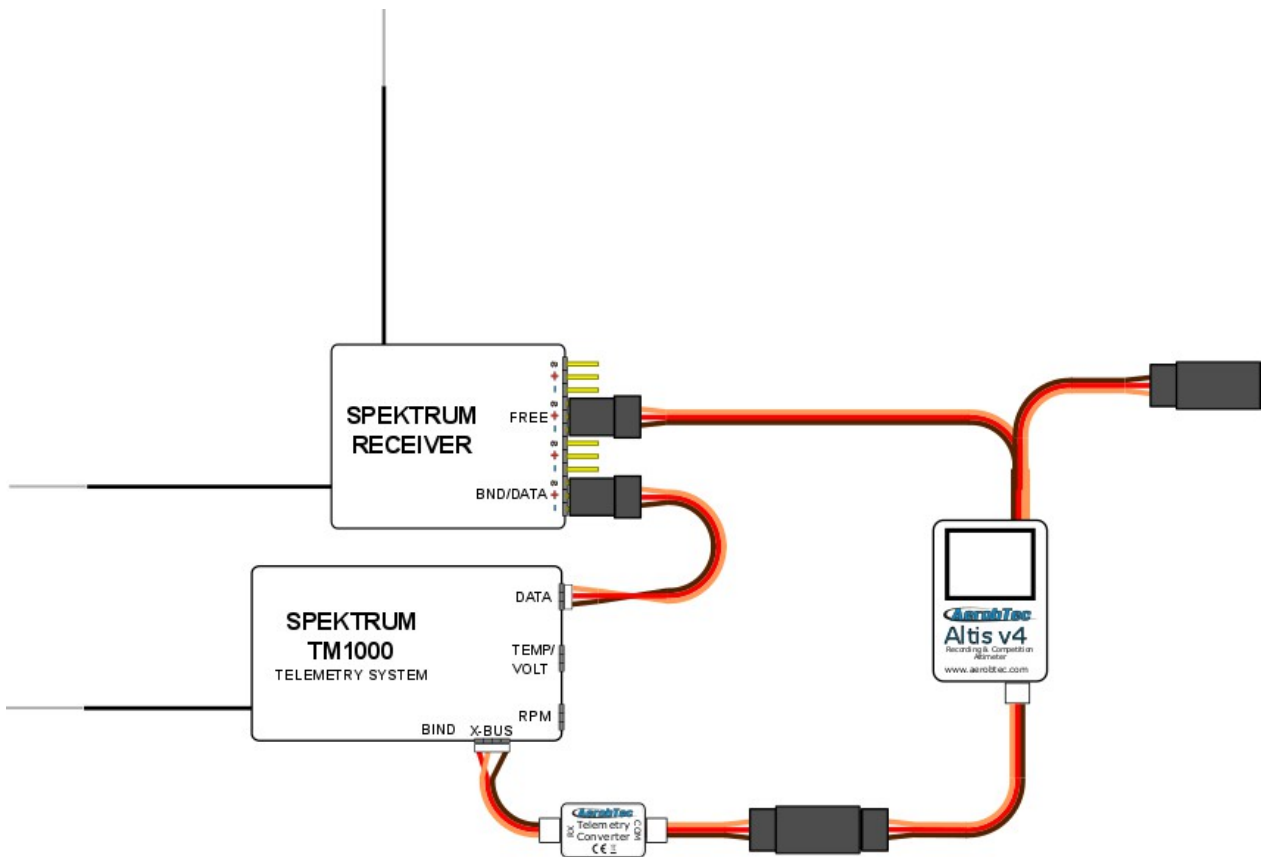
Fig. 3: Connection of the Telemetry Converter with Spektrum
